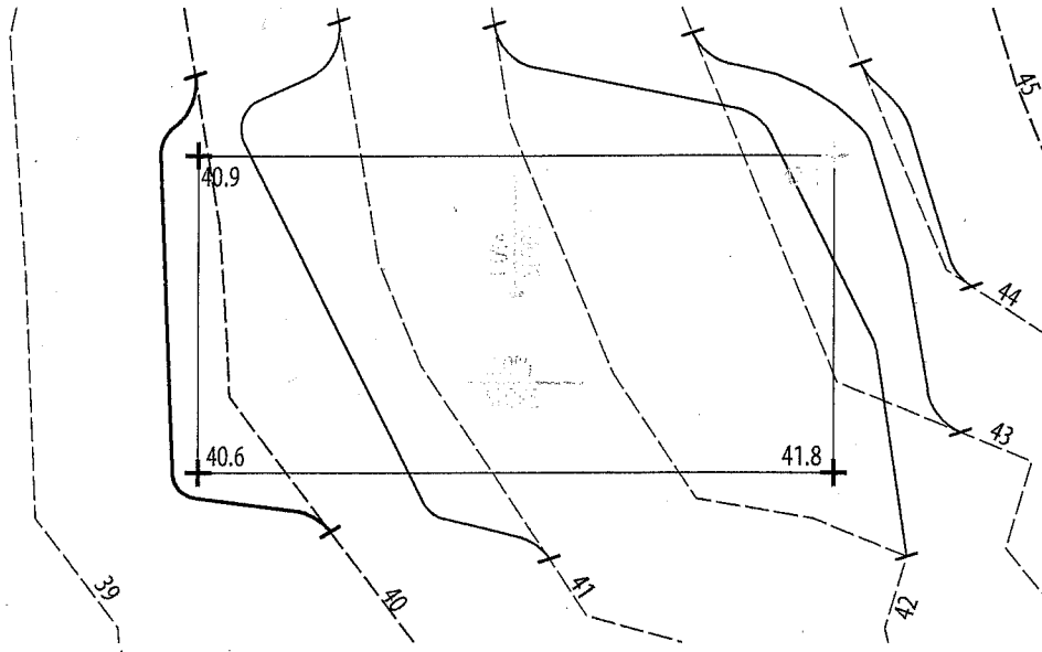
Figure 5.10A. Solution for terrace grading plan
